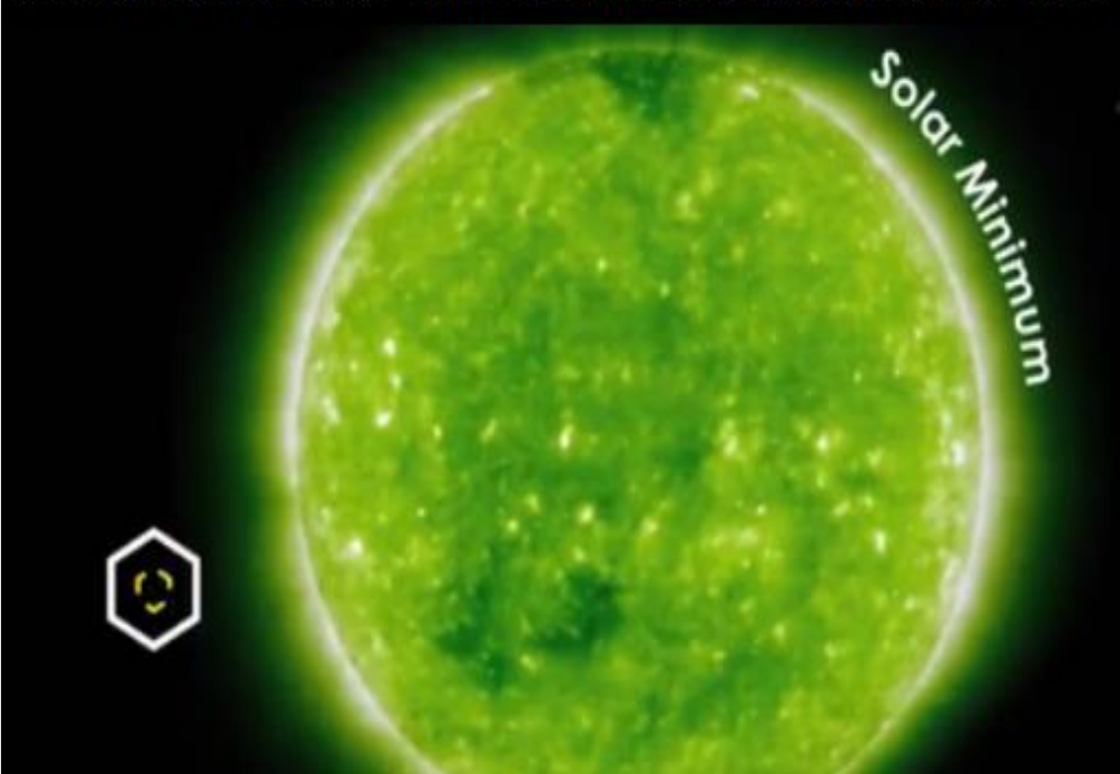
NASA predicts solar minimum will be at its lowest by 2020
